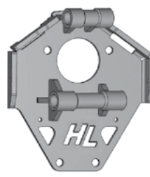
132o-L Left Rear Portal Backing Plate (1ea)
